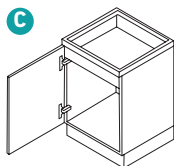
Spülenschrank Höhe = 723 mm Breite = 400, 450, 500, 600 mm 1 Drehtür Sink cabinet Height = 723 mm Width = 400, 450, 500, 600 mm 1 hinge door
