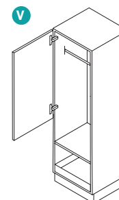
Garderobenschrank Höhe = 1907, 2051, 2195 mm Breite = 600 mm 2 feste Böden 1 Kleiderstange 1 Innenschubkasten Wardrobe Height = 1907, 2051, 2195 mm Width = 600 mm 2 fixed shelves 1 clothes rail 1 internal drawer
